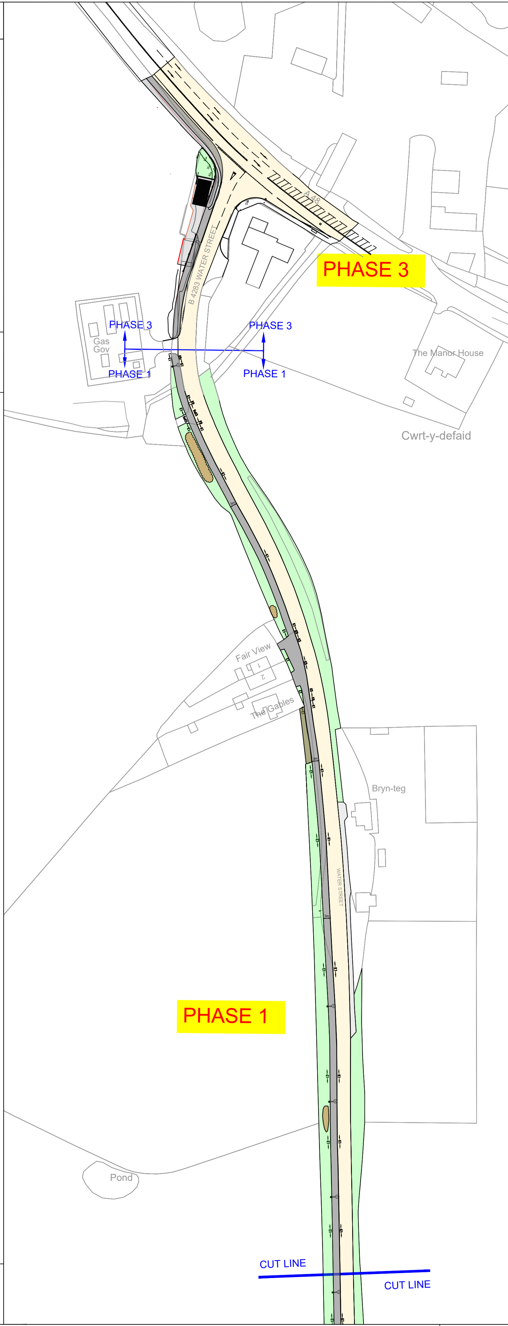
LAYOUT PLANS SCALE 1:1000
