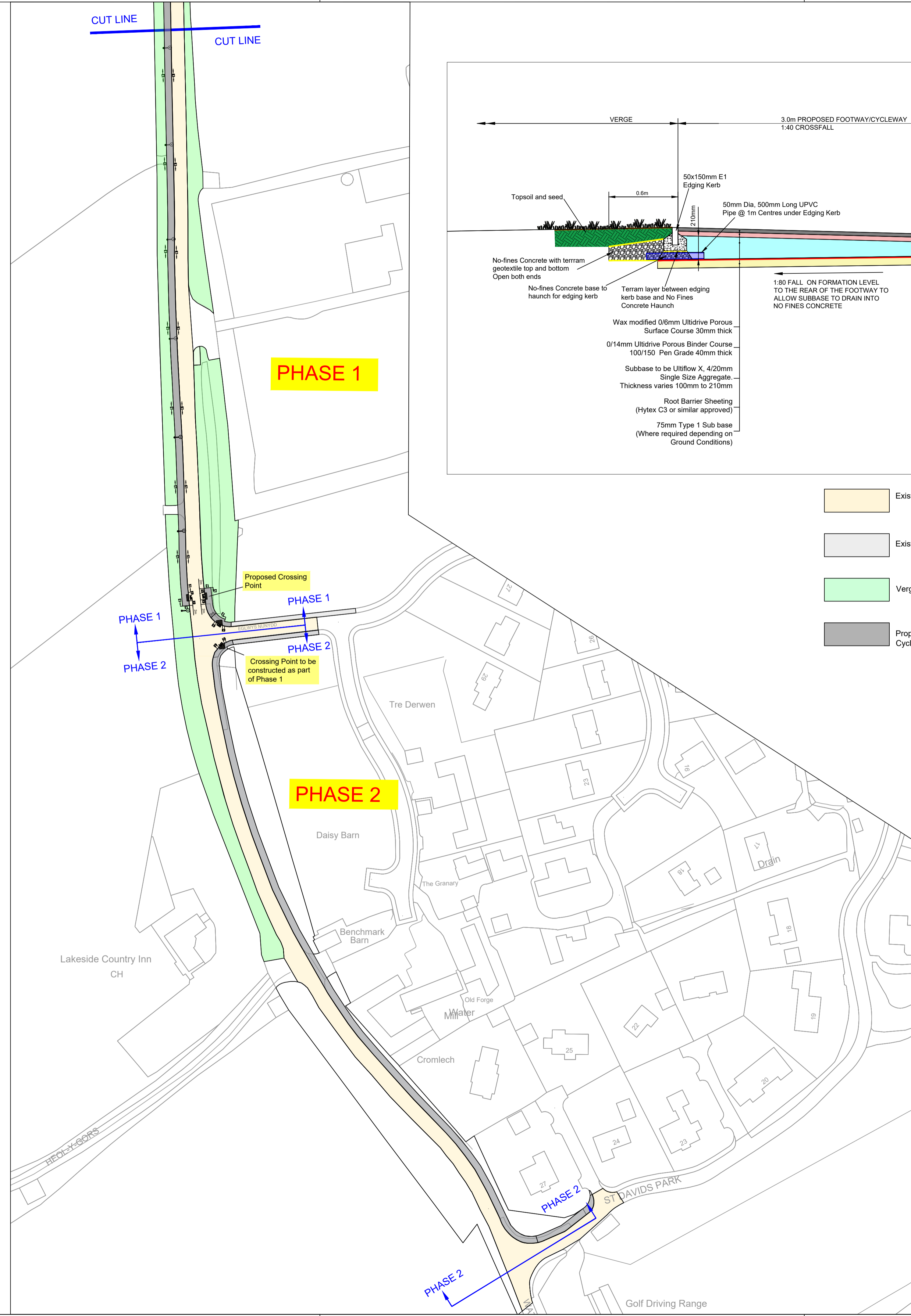
LAYOUT PLANS SCALE 1:1000
